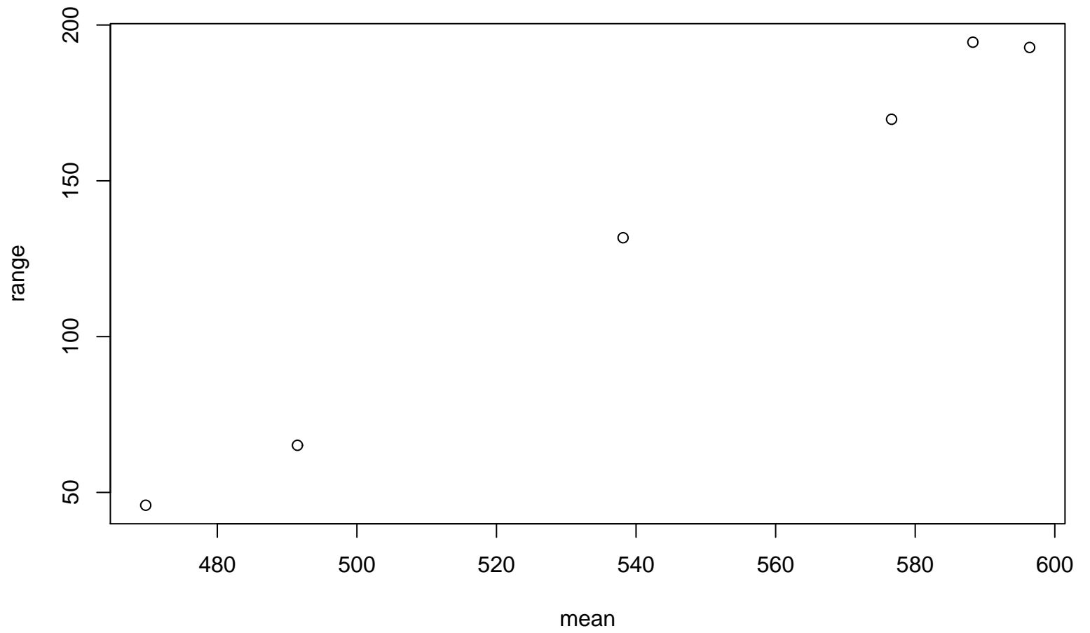
Range-Mean Plot
