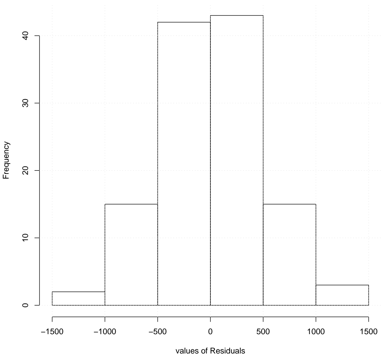
Residual Histogram
