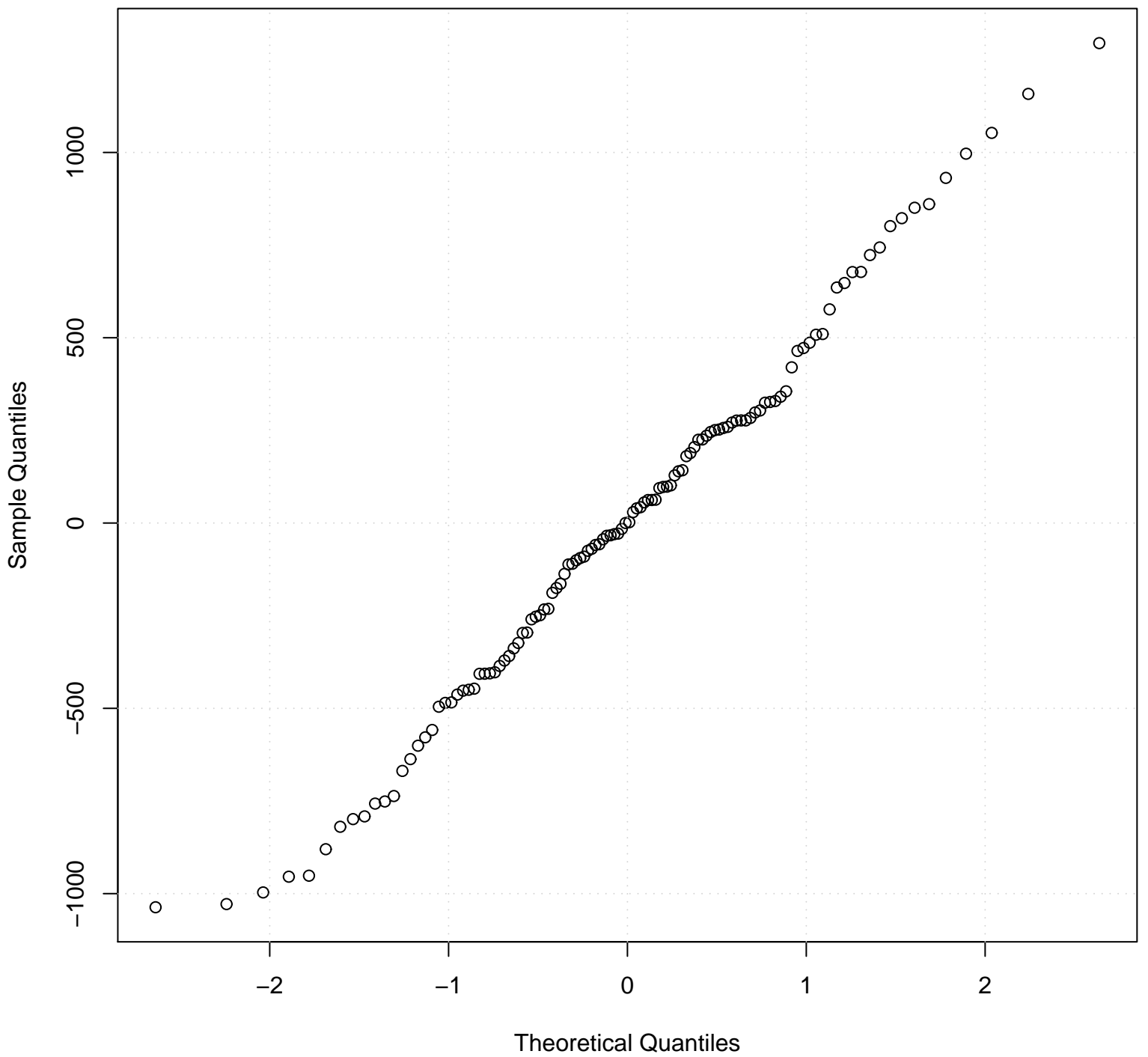
Residual Normal Q-Q Plot
