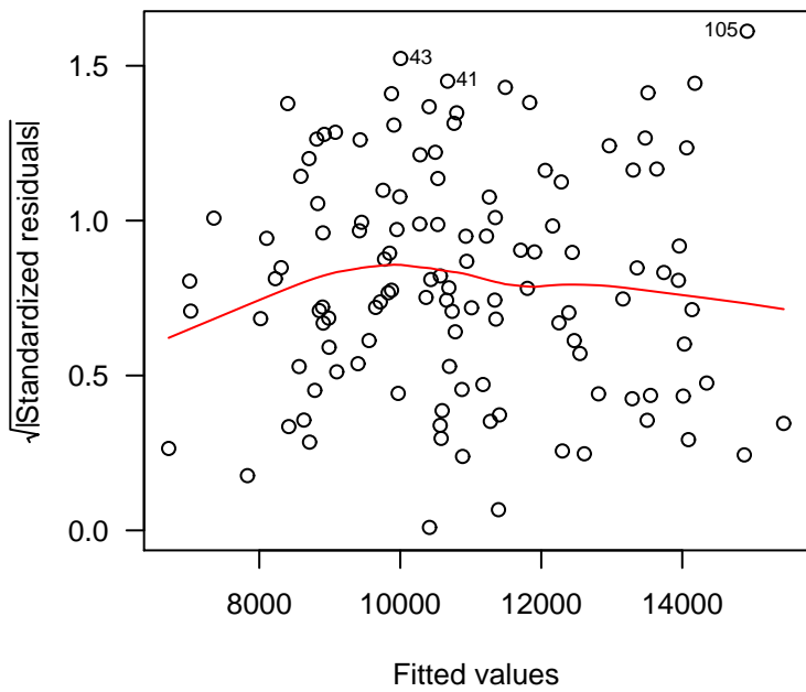
Scale-Location
