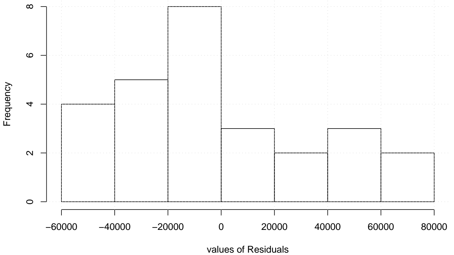
Residual Histogram
