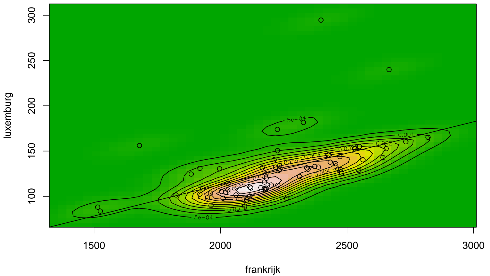
Bivariate Kernel Density(invoer)
