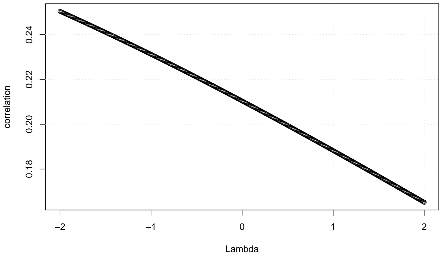
Box-Cox Linearity Plot
