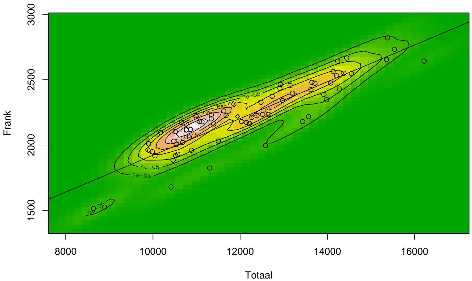
Bivariate Kernel Density(invoer)
