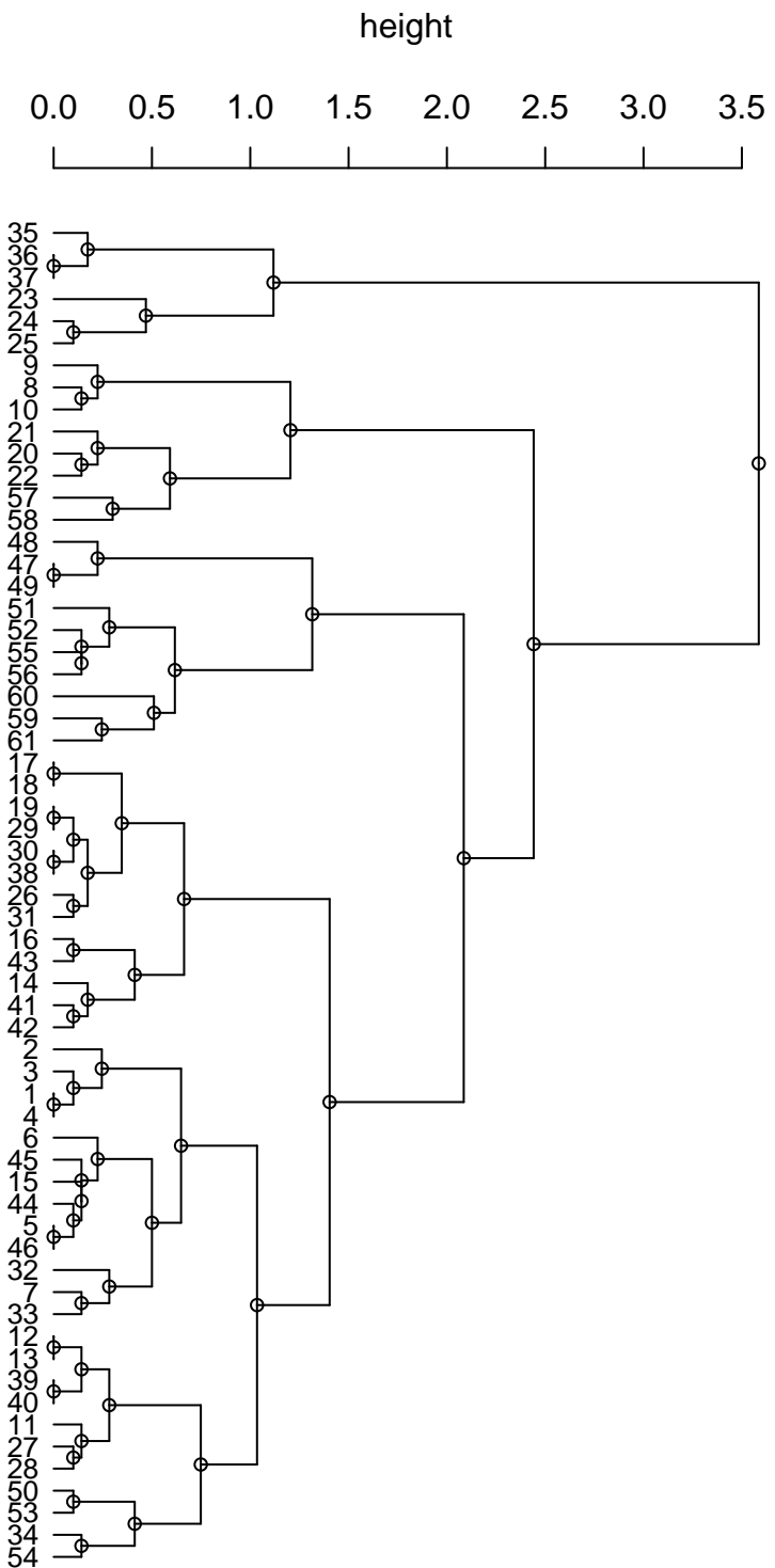
Dendrogram
