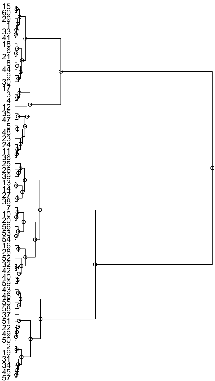
Dendrogram
