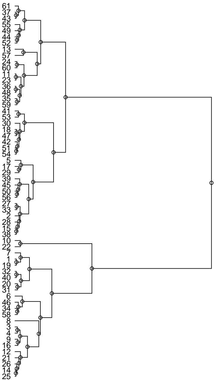
Dendrogram
