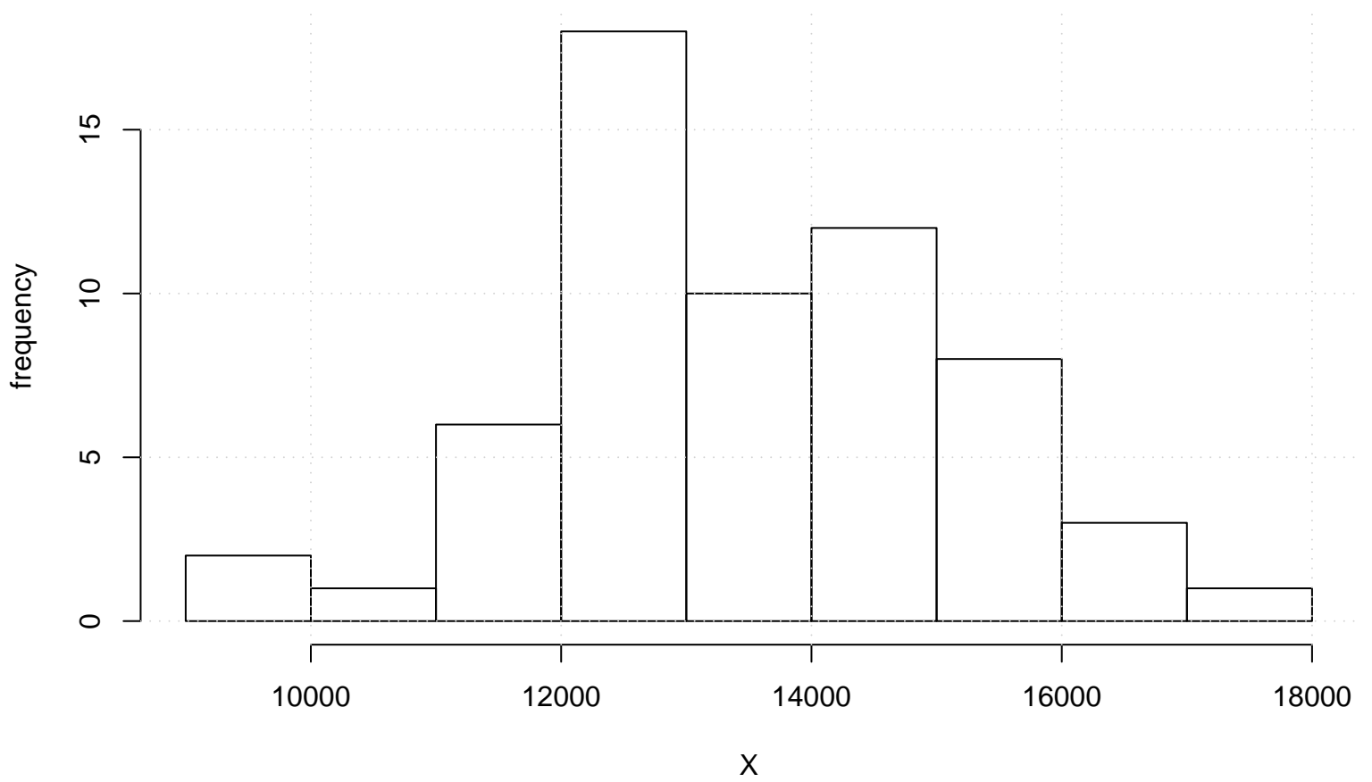
Histogram of Original Data
