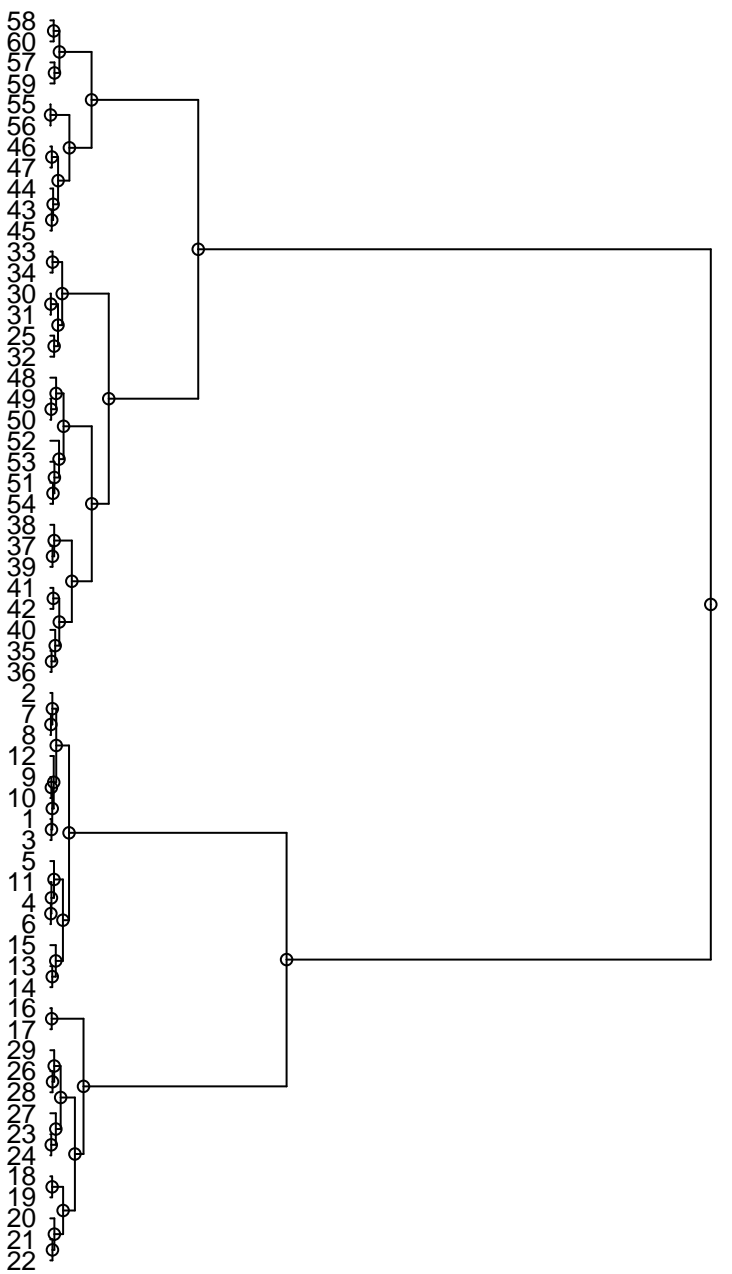
Dendrogram
