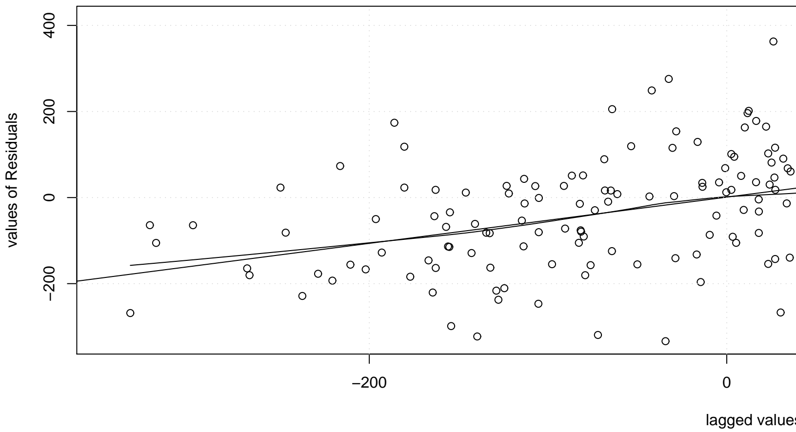
Residual Lag plot, lower
