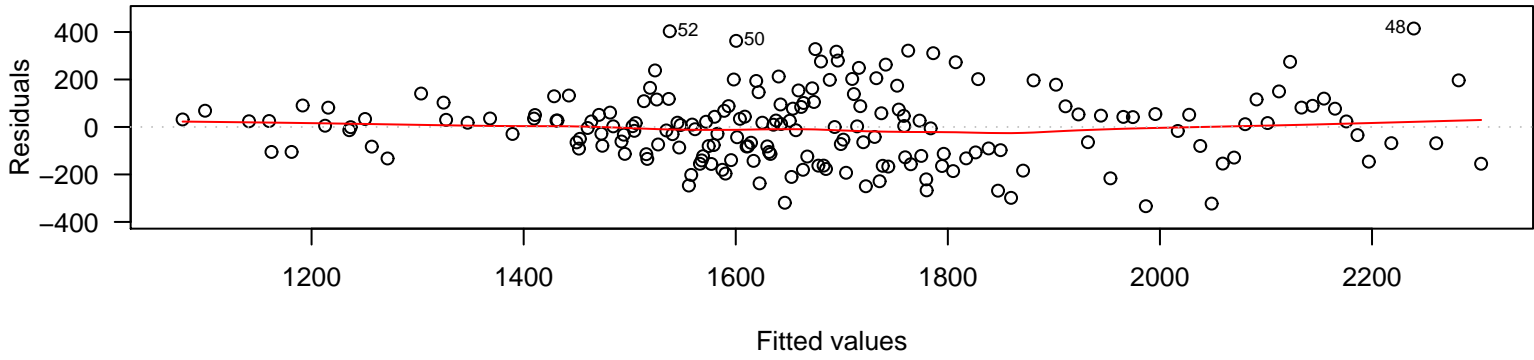
Residuals vs Fitted
