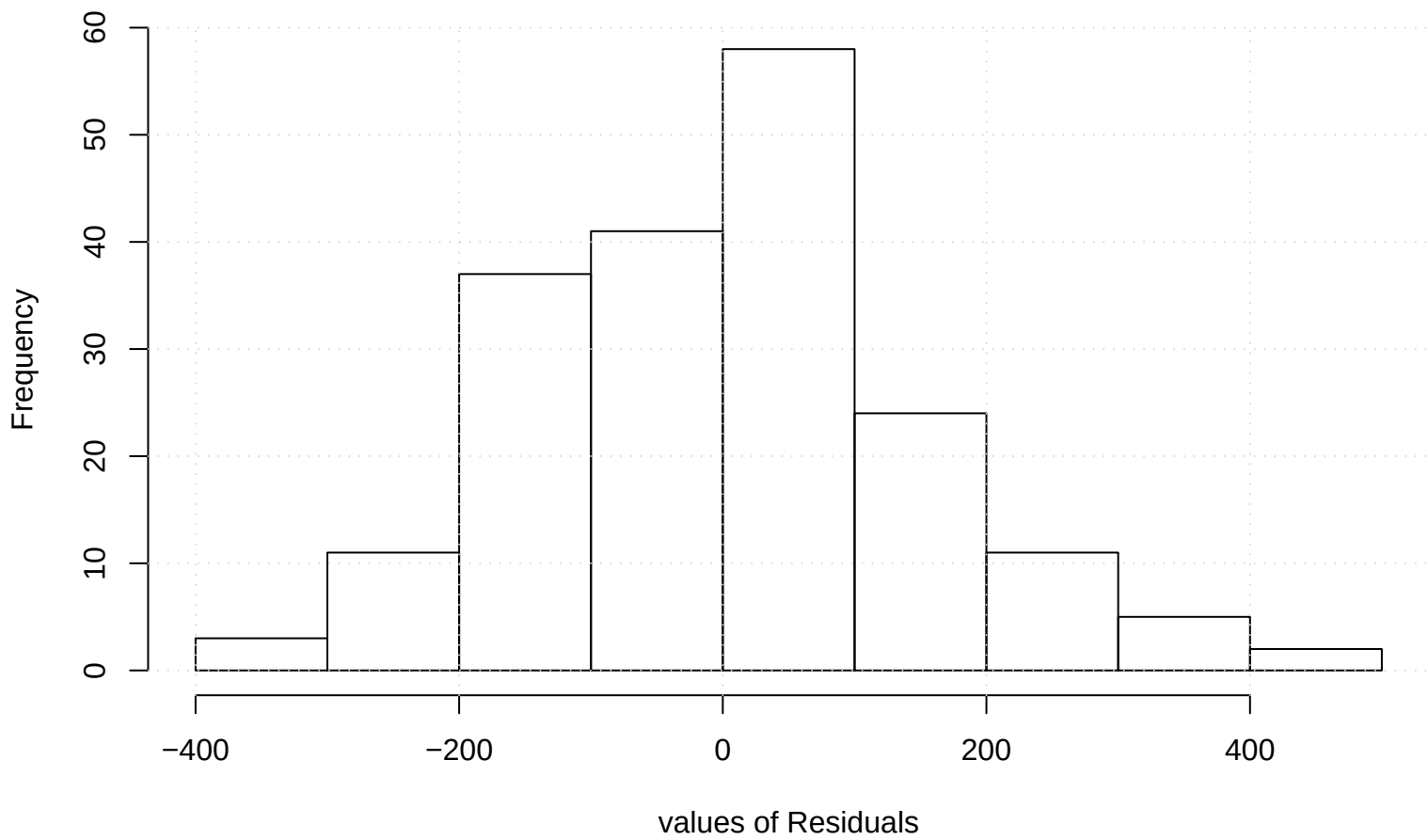
Residual Histogram
