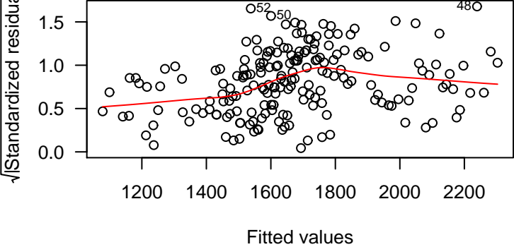
Scale-Location
