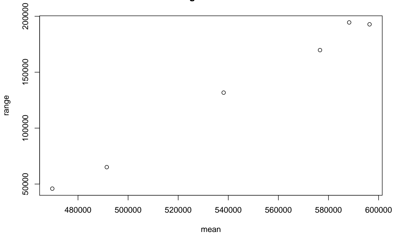
Range-Mean Plot
