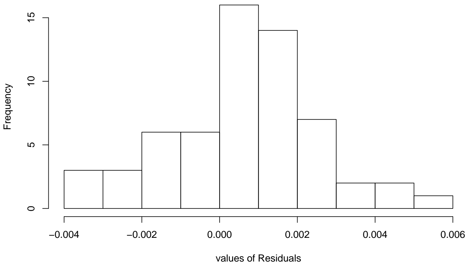
Residual Histogram
