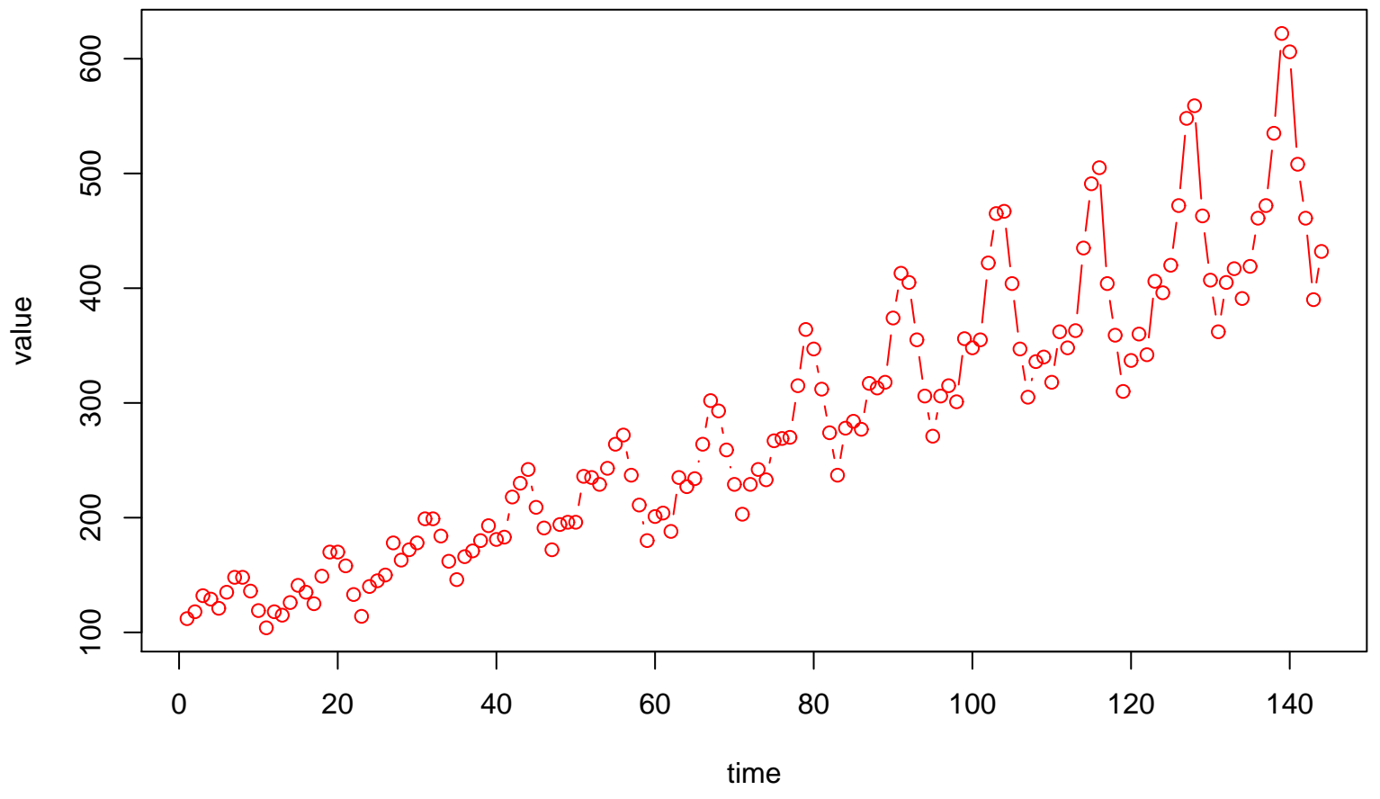
Airline data
