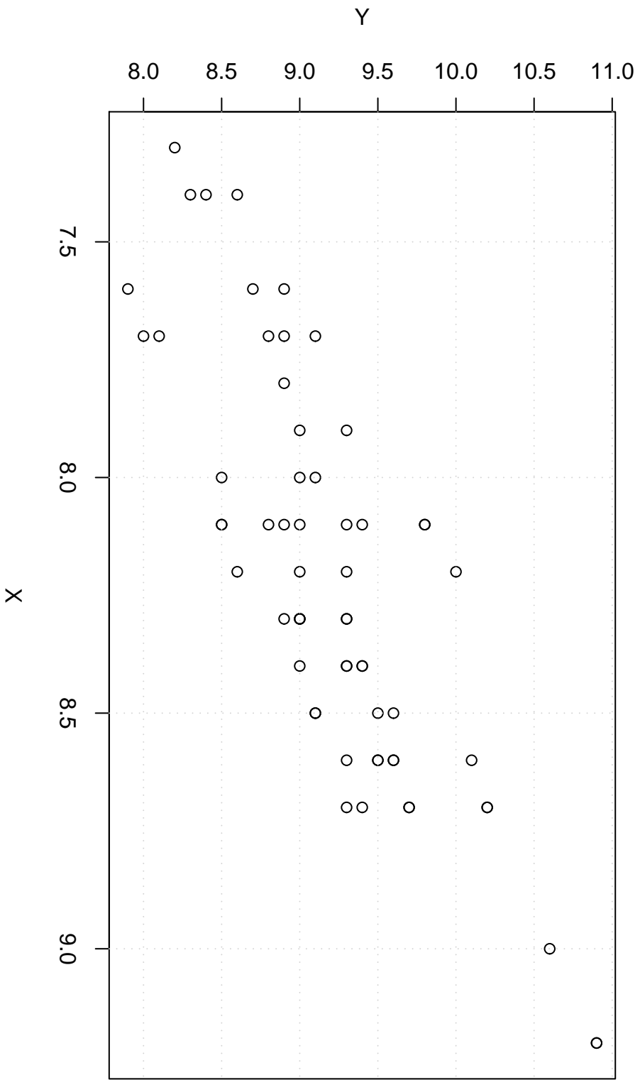
Scatterplot
