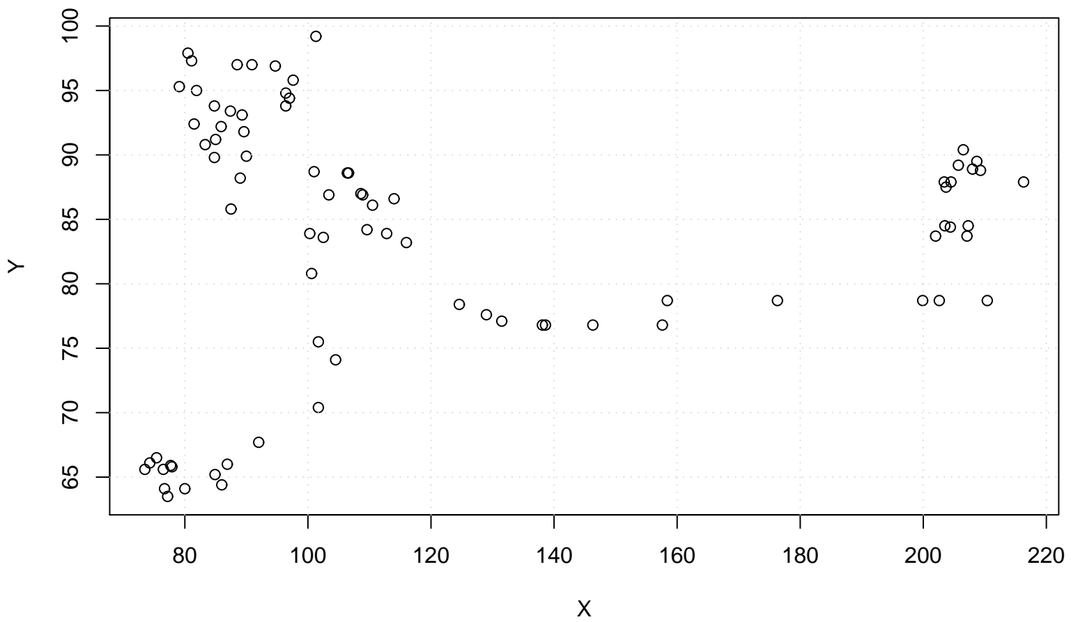
Scatterplot
