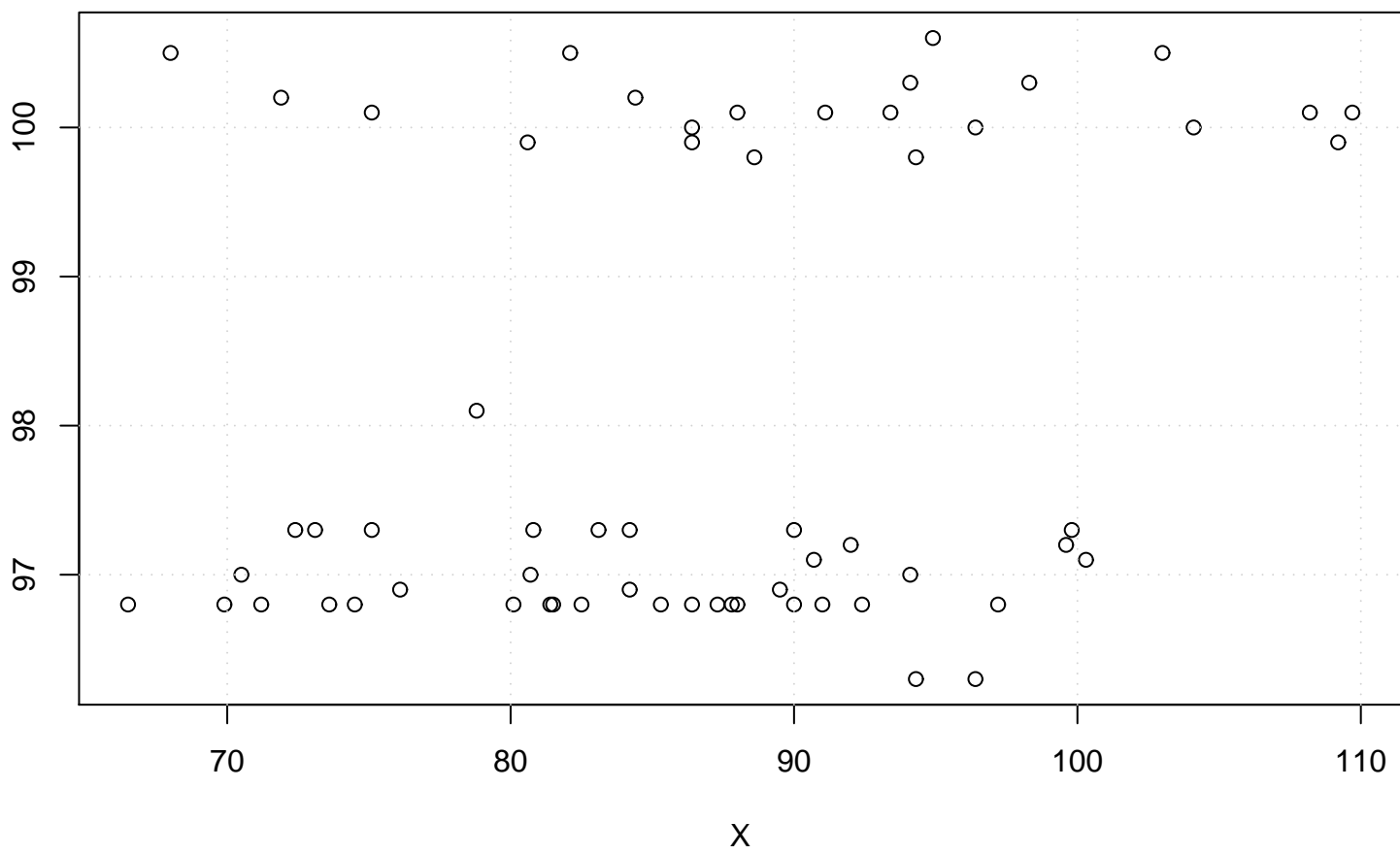
Scatterplot
