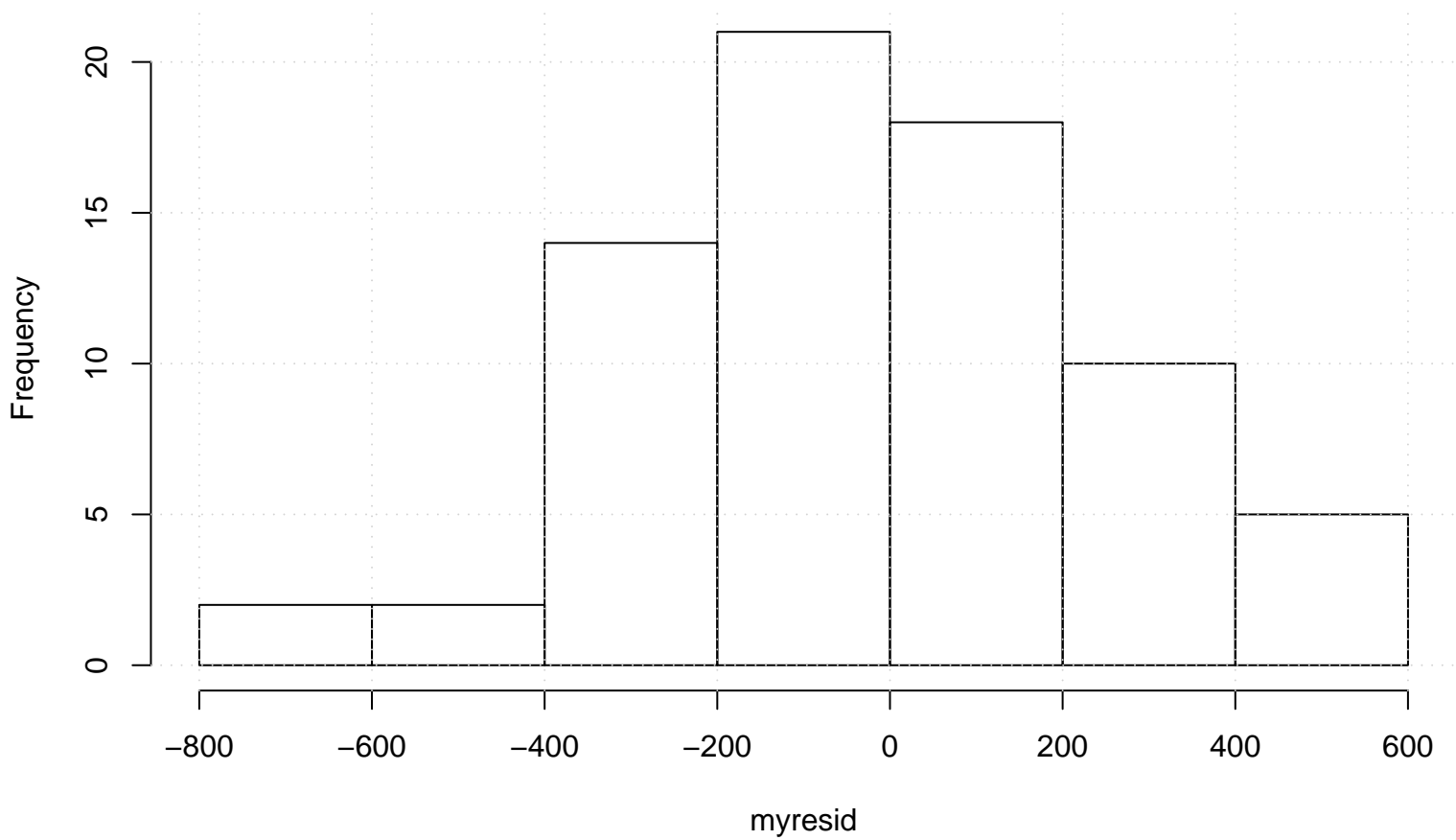
Histogram of myresid
