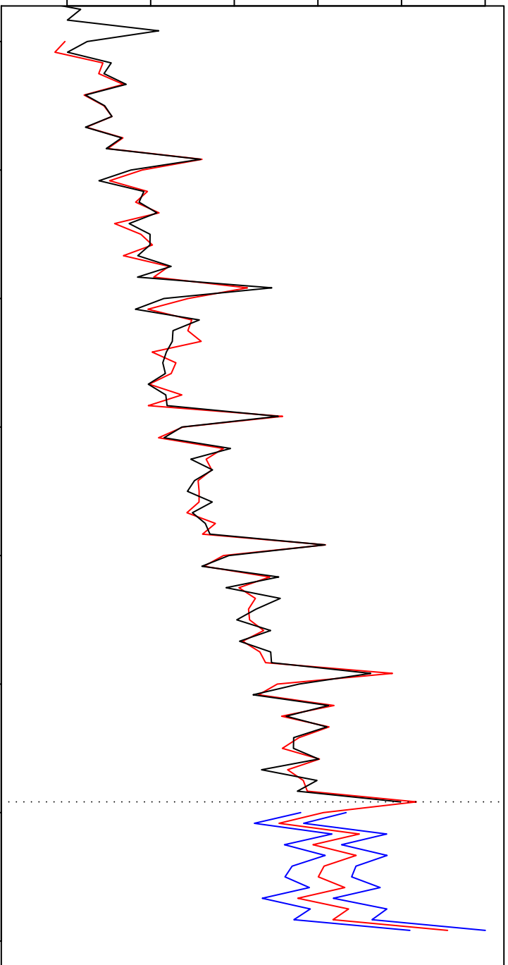
Extrapolation Fit of Exponential Smoothing
