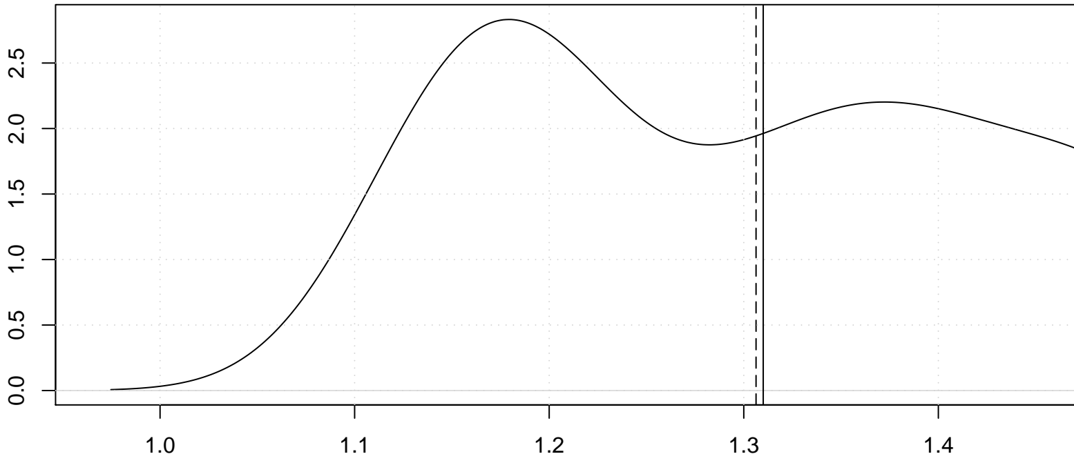
Density Plot – Gaussian Kernel
