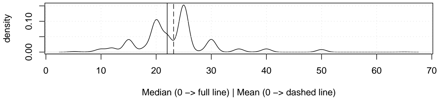
Density Plot – Gaussian Kernel
