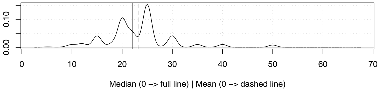
Density Plot – Gaussian Kernel
