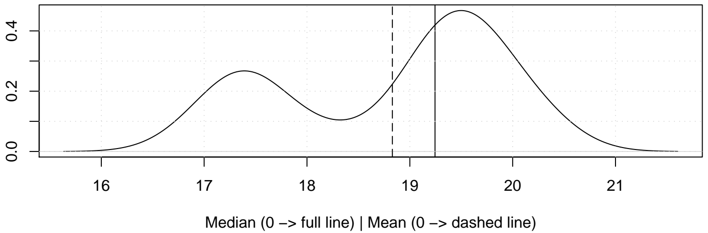
Density Plot – Gaussian Kernel
