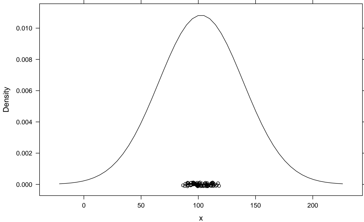
Density Plot bw = 36
