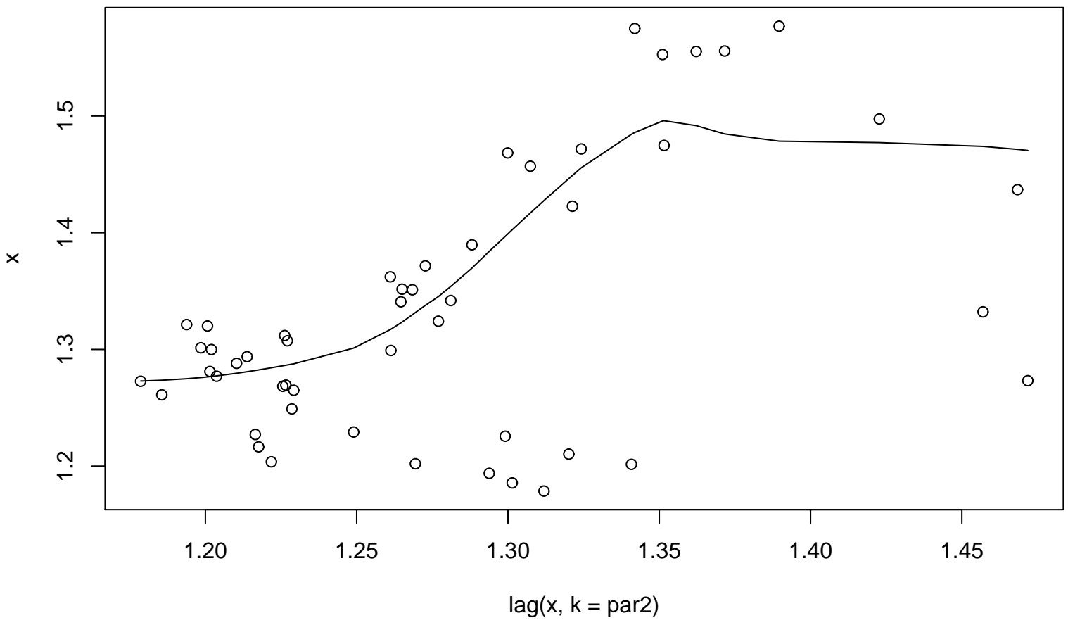
Lag plot (k=10), and lowess
