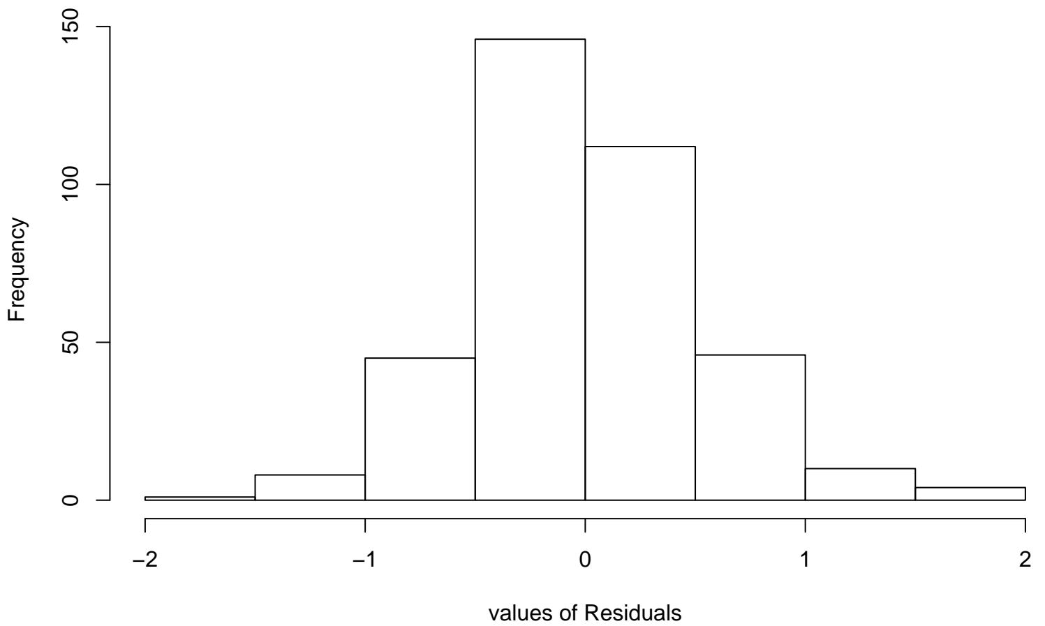
Residual Histogram
