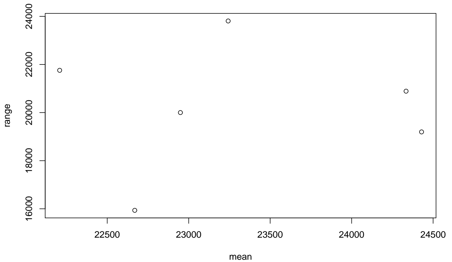
Range-Mean Plot
