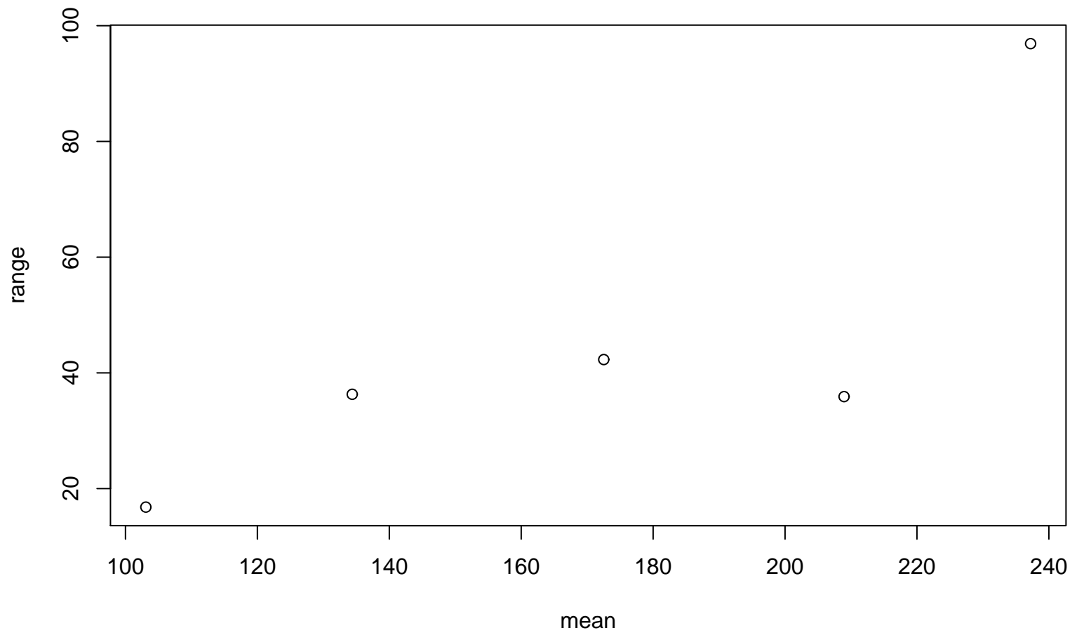
Range-Mean Plot
