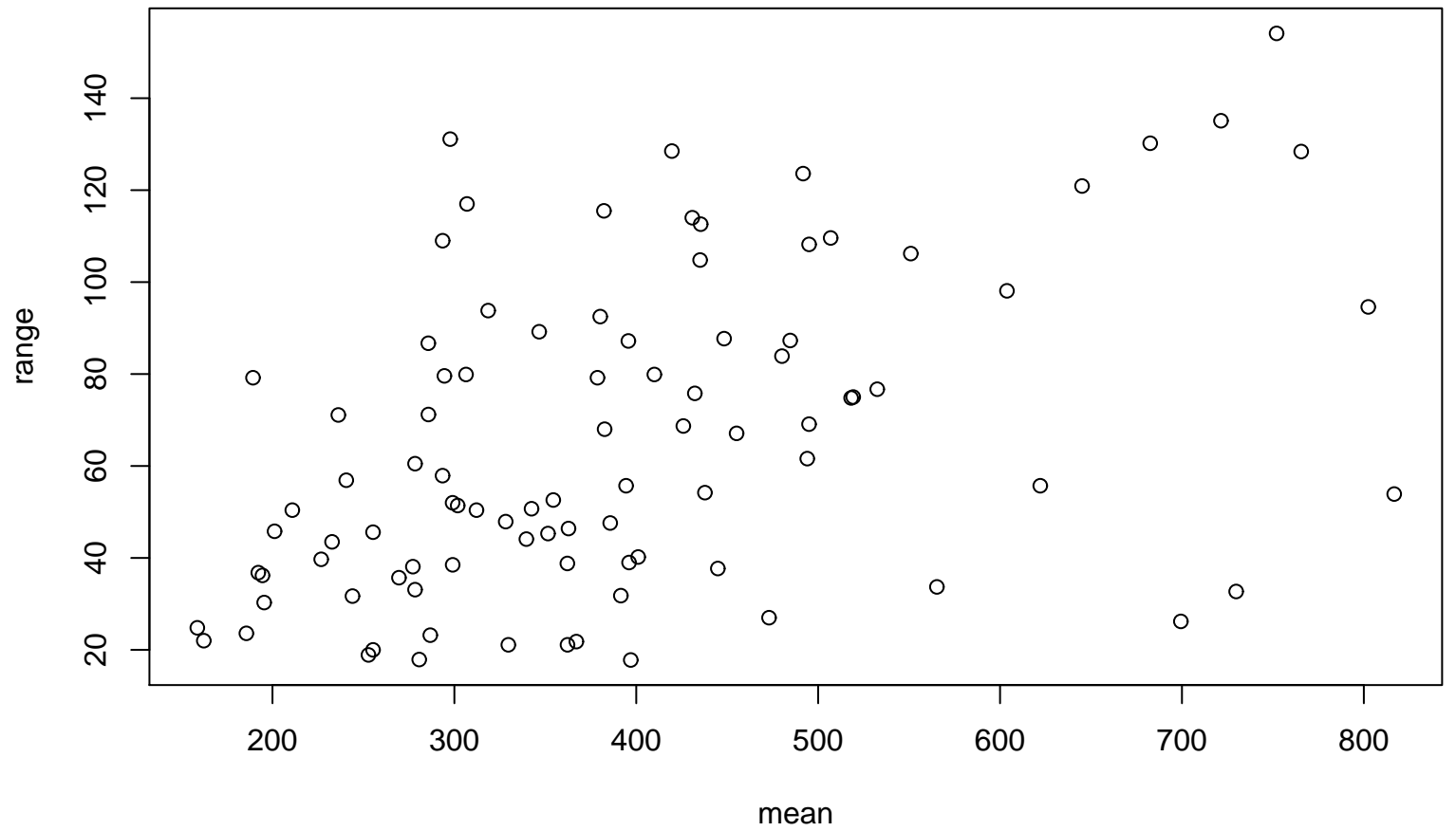
Range-Mean Plot
