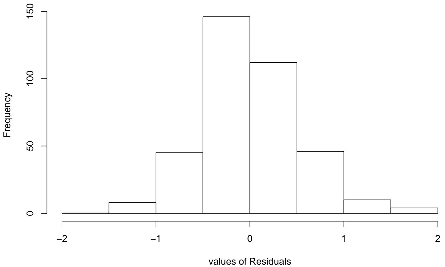
Residual Histogram
