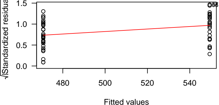
Scale-Location
