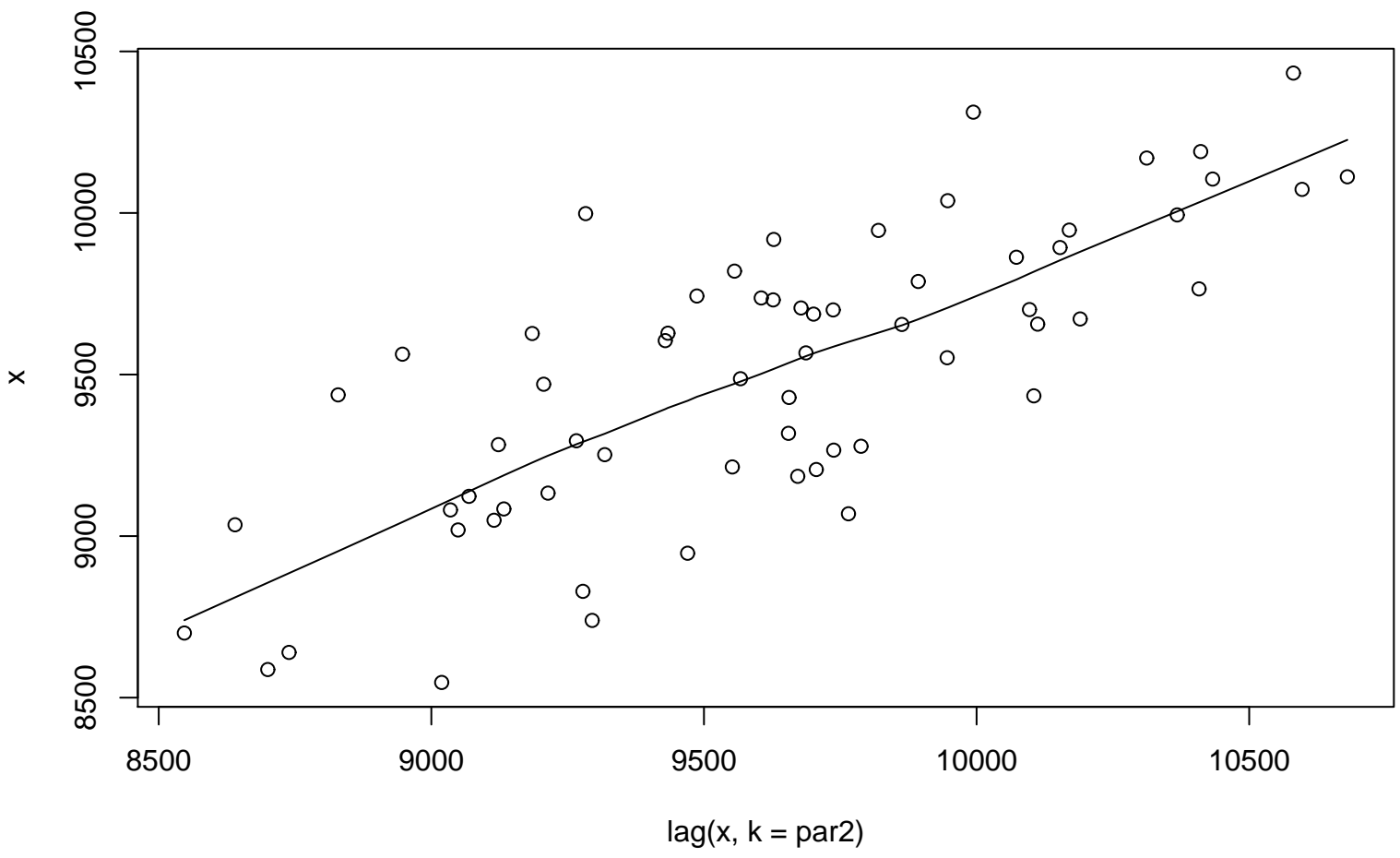
Lag plot (k=12), and lowess
