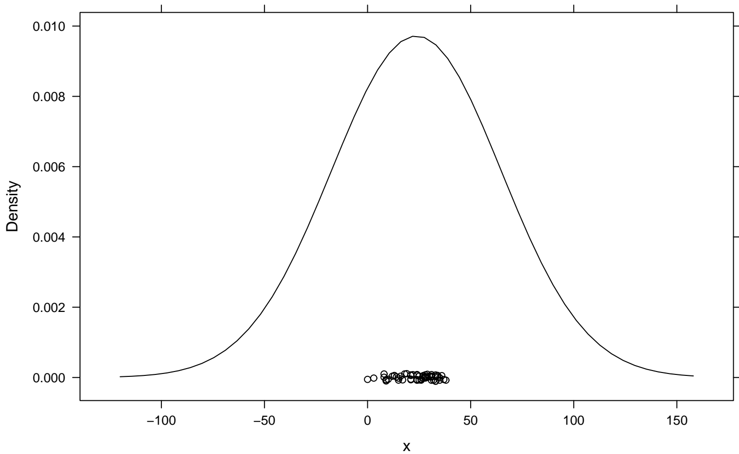
Density Plot bw = 40
