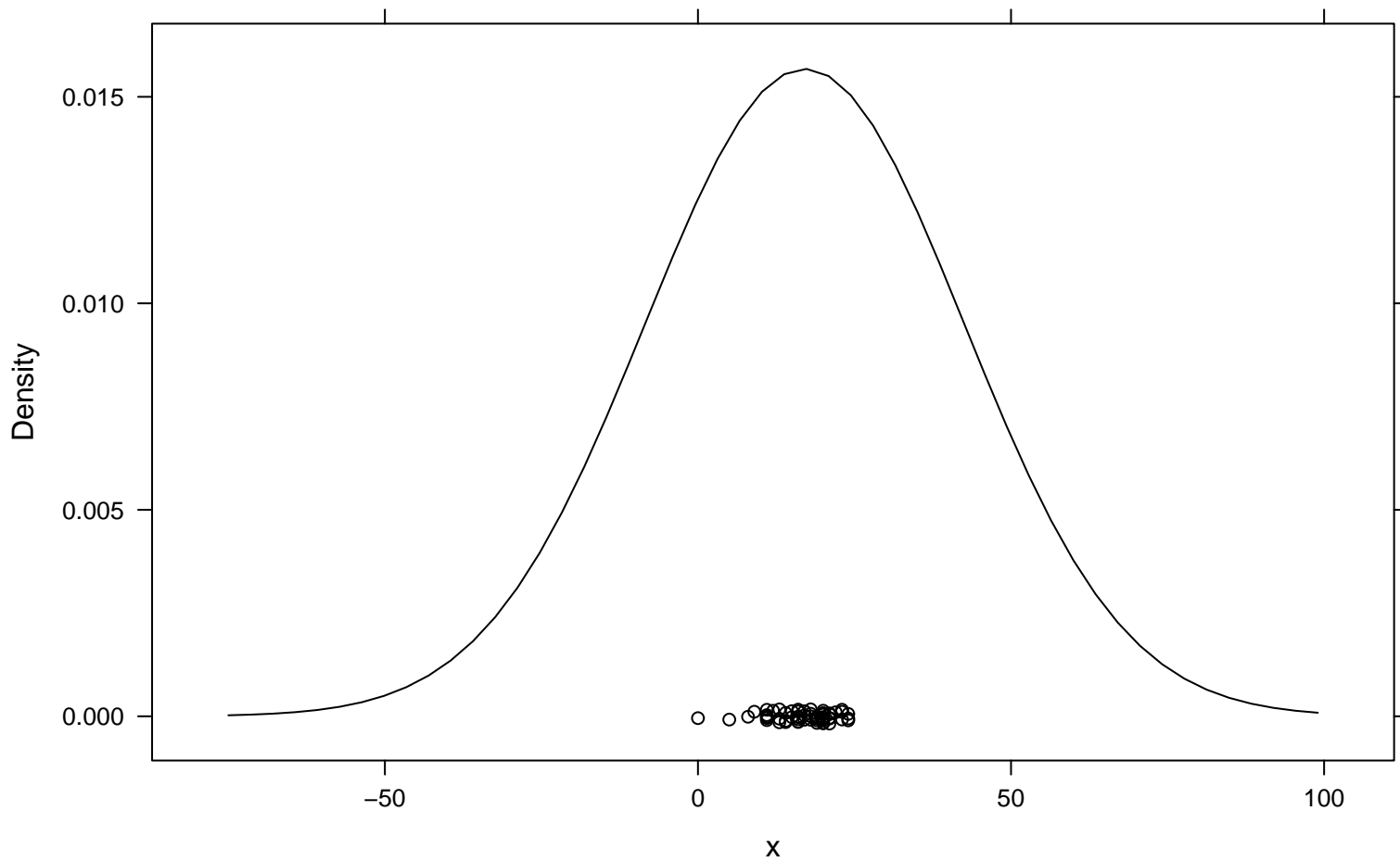
Density Plot bw = 25
