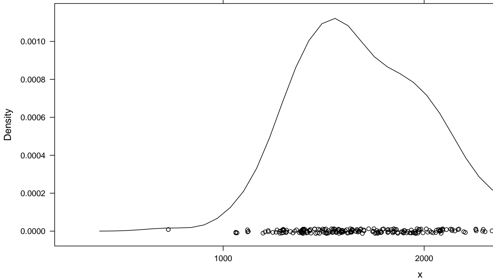
Density Plot
