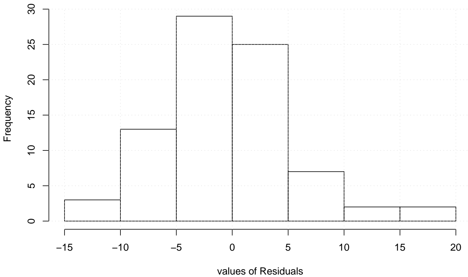
Residual Histogram
