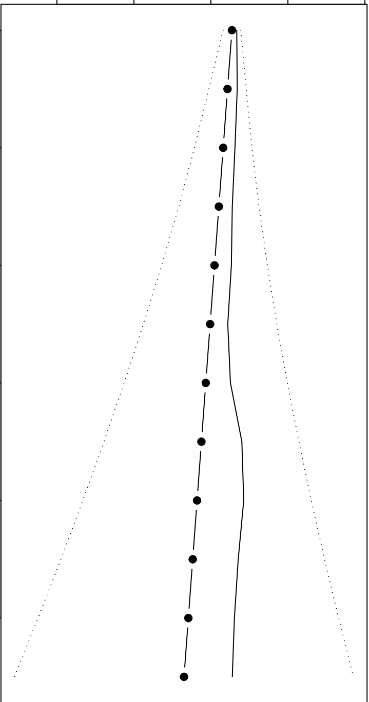
ARIMA Extrapolation Forecast
