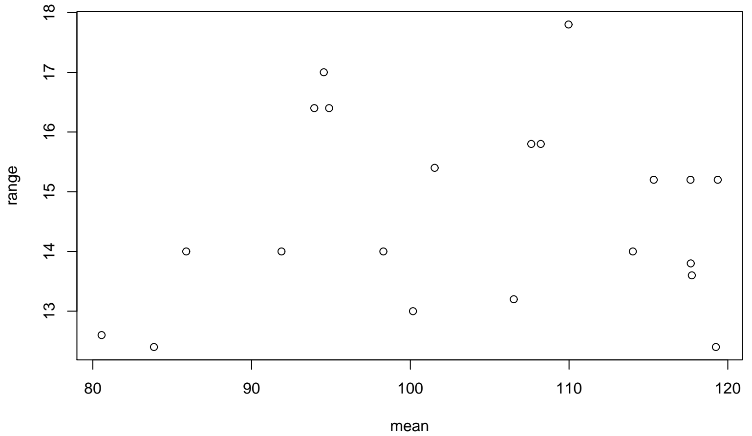
Range-Mean Plot
