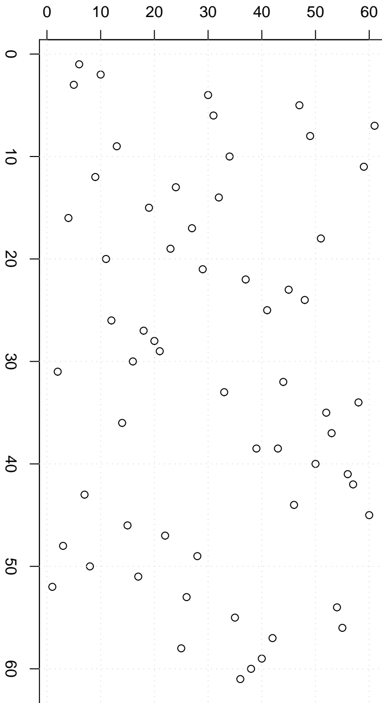
Scatterplot of Ranks
