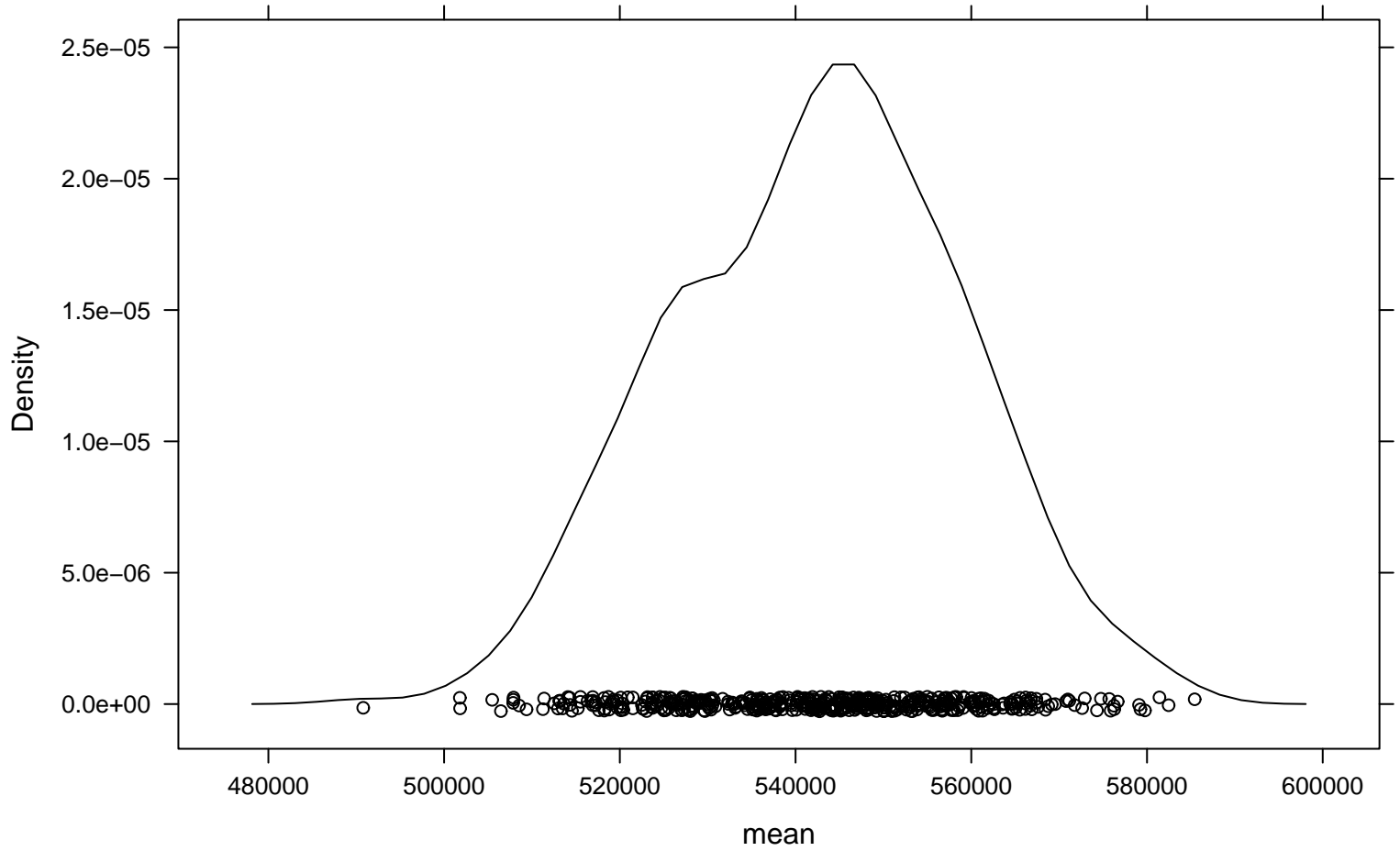
Density Plot
