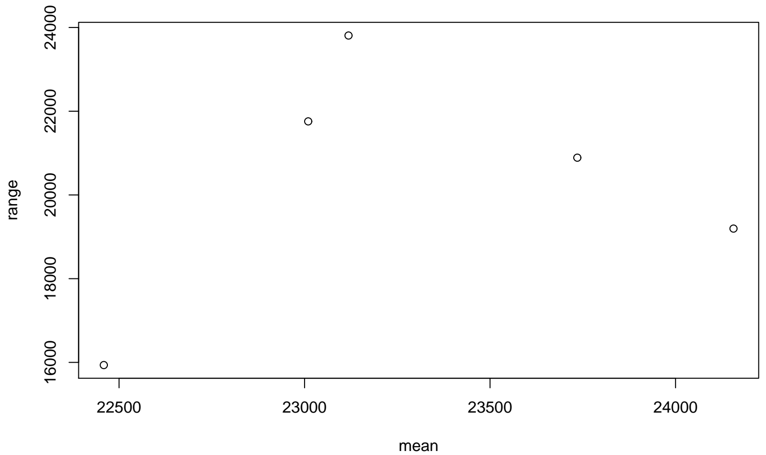
Range-Mean Plot
