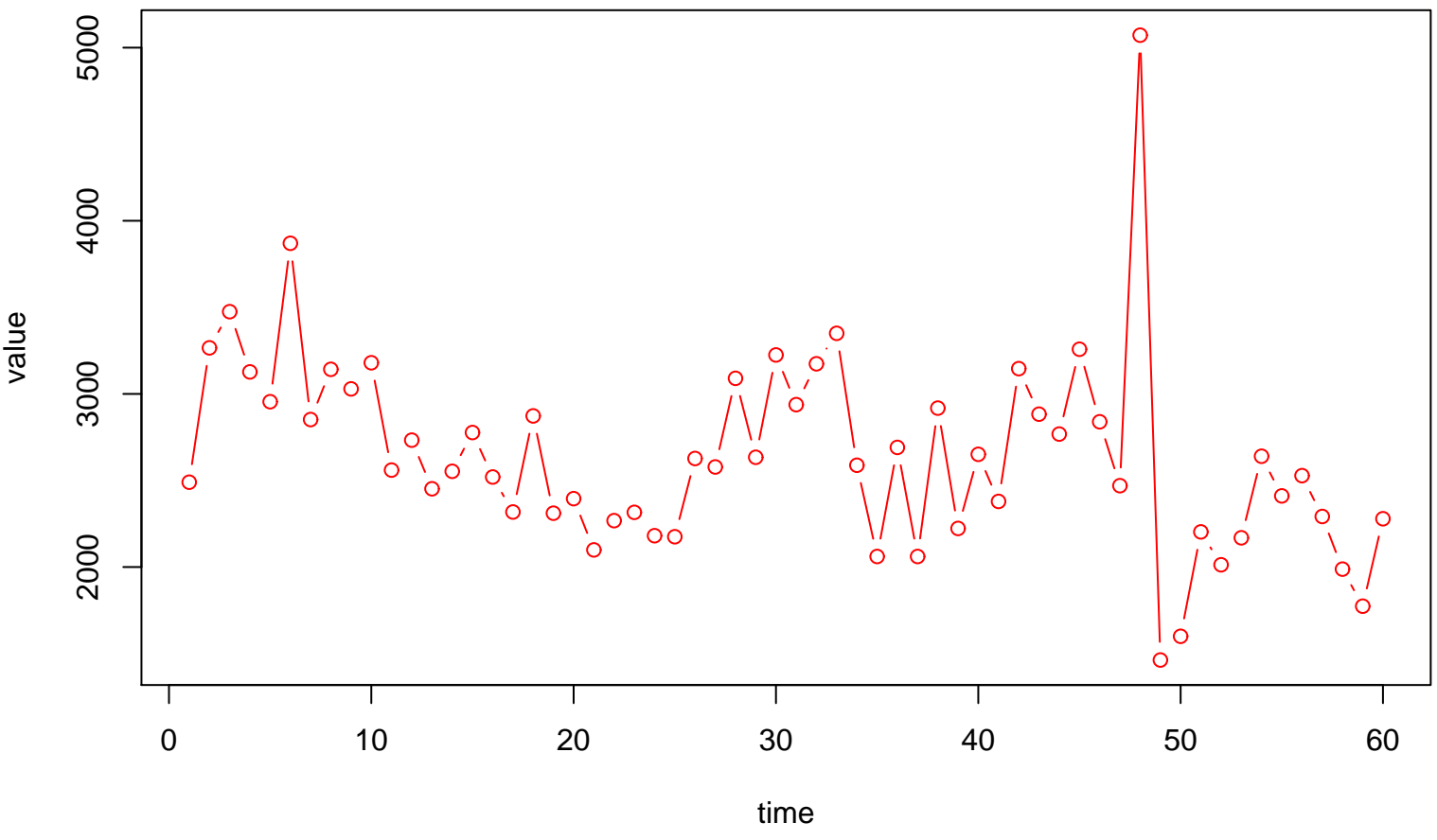
Run-Sequence Plot
