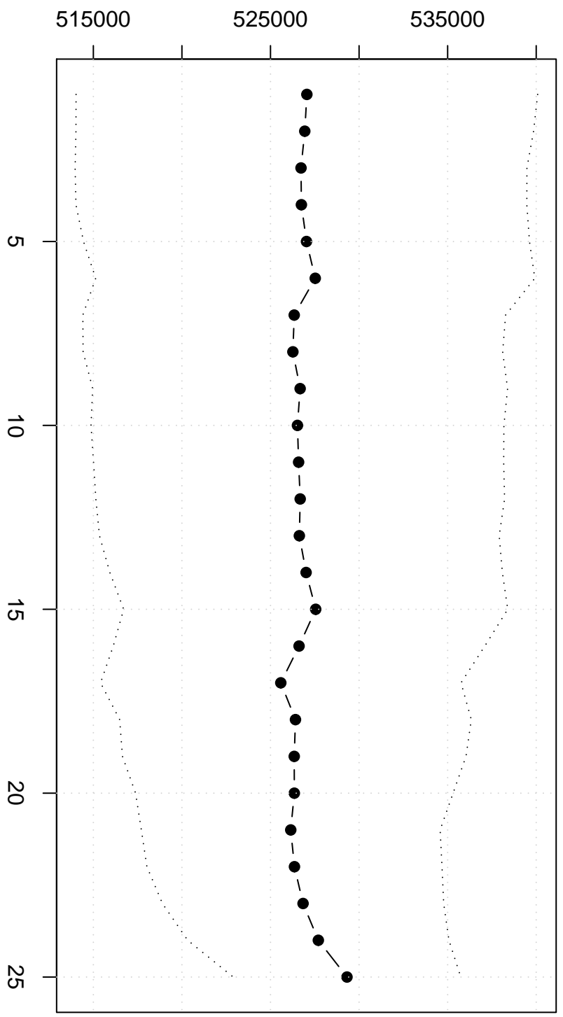
Winsorized Mean(j/n)
