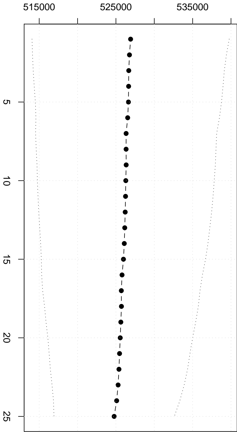
Trimmed Mean( j/n )
